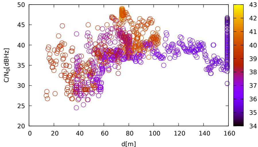
C/N 0 vs distance (TrimbleR10 at C 2 for G32 at L1)
