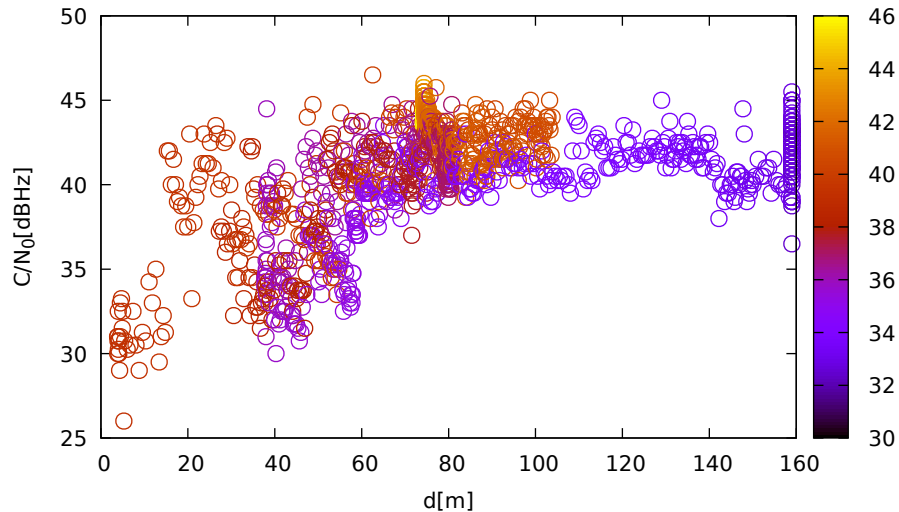
C/N 0 vs distance (TrimbleR10 at C 2 for R06 at L1)
