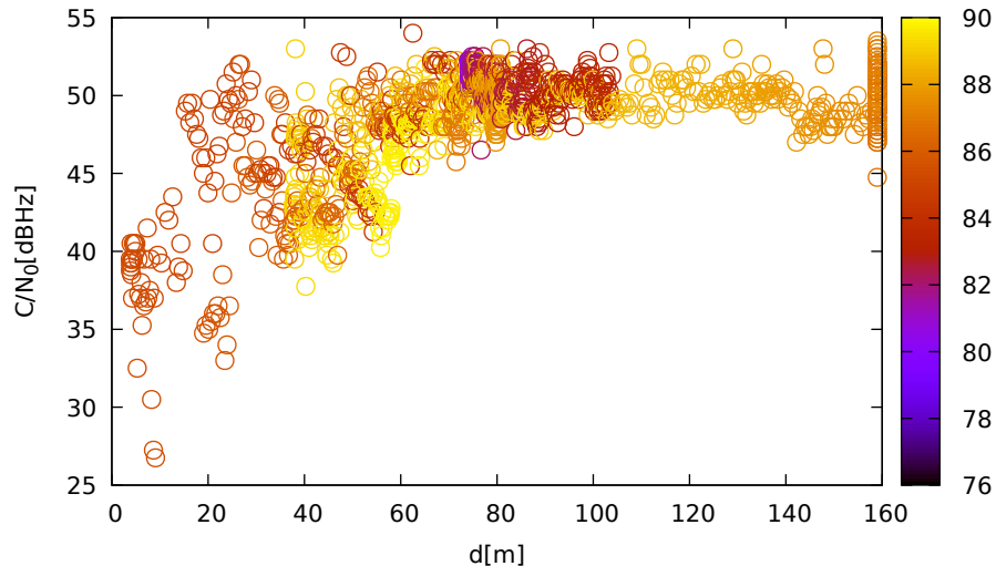
C/N 0 vs distance (TrimbleR10 at C 2 for R07 at L1)
