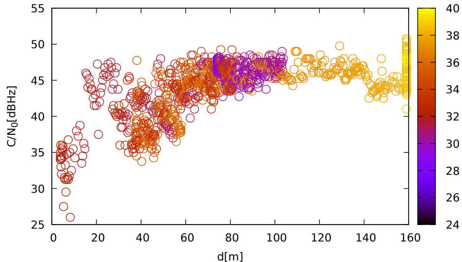
C/N 0 vs distance (TrimbleR10 at C 2 for R08 at L1)
