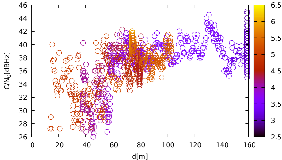
C/N 0 vs distance (TrimbleR10 at C 2 for R14 at L1)
