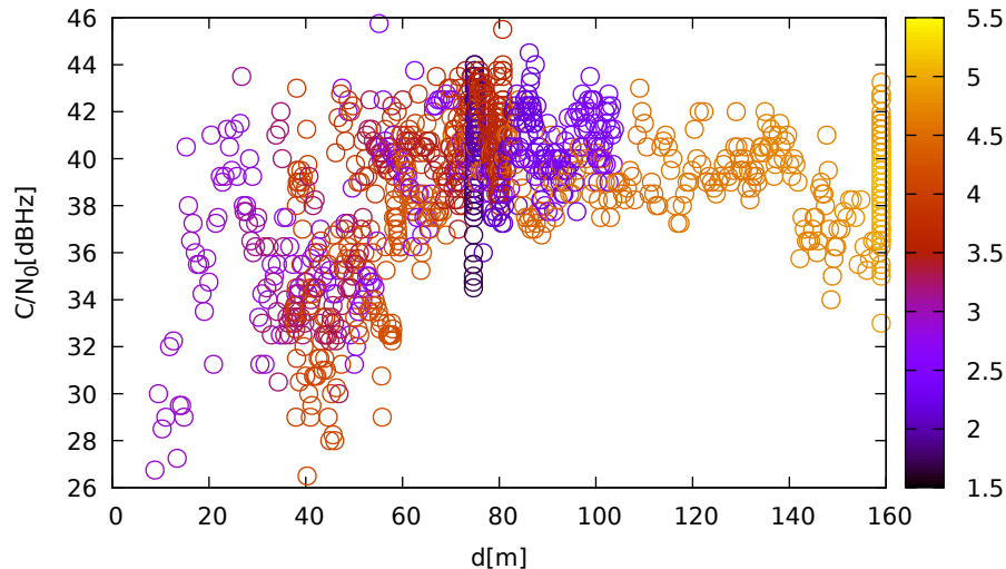
C/N 0 vs distance (TrimbleR10 at C 2 for R15 at L1)
