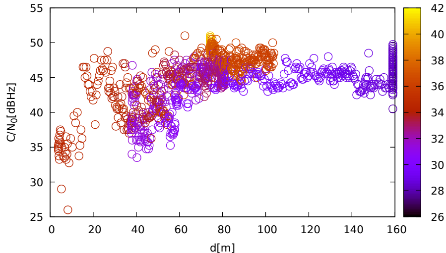
C/N 0 vs distance (TrimbleR10 at C 2 for R21 at L1)
