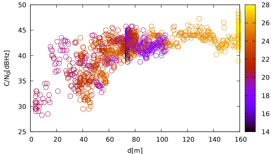
C/N 0 vs distance (TrimbleR10 at C 2 for R23 at L1)
