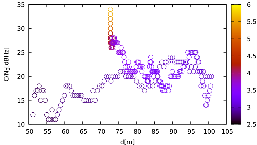
C/N 0 vs distance (ublox9 at C 2 for E02 at L1)
