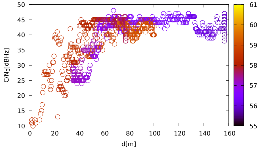
C/N 0 vs distance (ublox9 at C 2 for E04 at L1)
