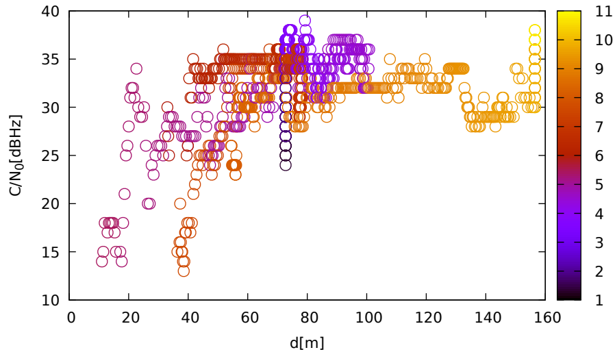
C/N 0 vs distance (ublox9 at C 2 for E05 at L1)
