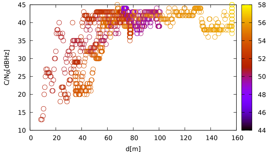
C/N 0 vs distance (ublox9 at C 2 for E09 at L1)
