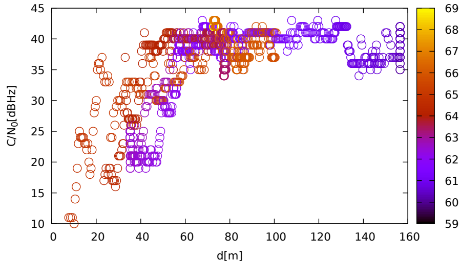
C/N 0 vs distance (ublox9 at C 2 for E11 at L1)
