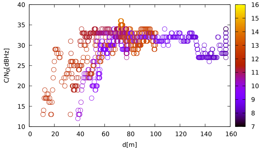
C/N 0 vs distance (ublox9 at C 2 for E12 at L1)
