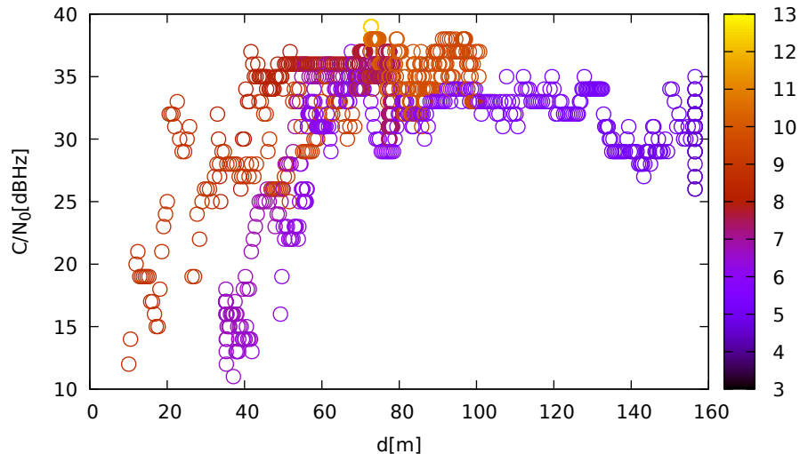
C/N 0 vs distance (ublox9 at C 2 for E19 at L1)
