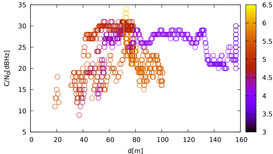
C/N 0 vs distance (ublox9 at C 2 for E30 at L1)
