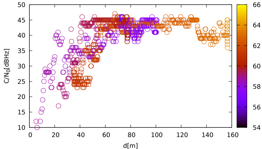
C/N 0 vs distance (ublox9 at C 2 for E36 at L1)
