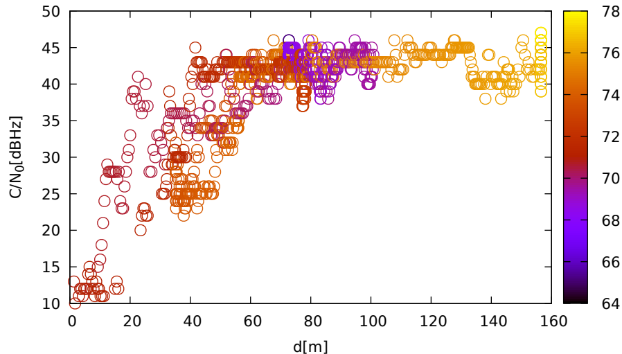
C/N 0 vs distance (ublox9 at C 2 for G01 at L1)
