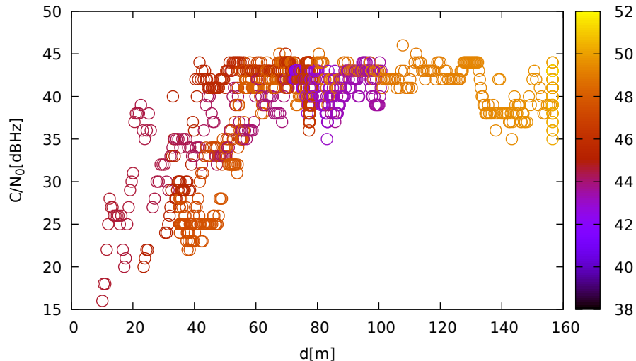
C/N_0 vs distance (ublox9 at C_2 for G03 at L1)
