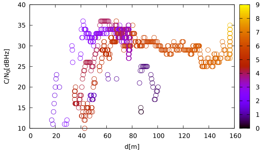
C/N 0 vs distance (ublox9 at C 2 for G04 at L1)
