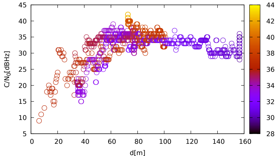
C/N_0 vs distance (ublox9 at C_2 for G08 at L1)
