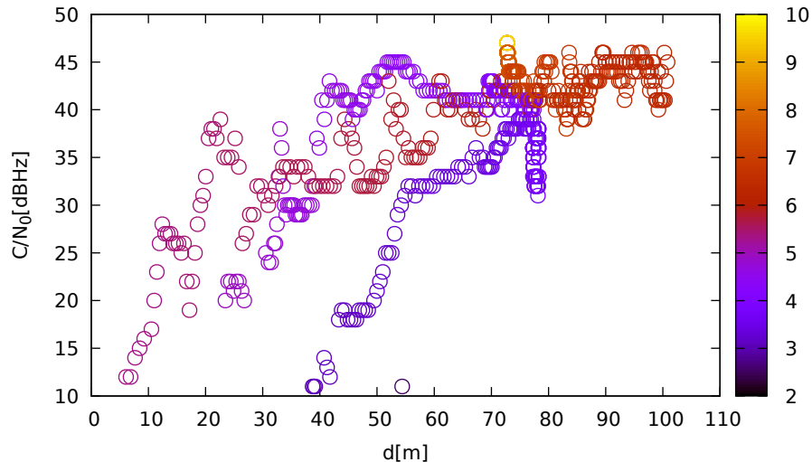
C/N 0 vs distance (ublox9 at C 2 for G10 at L1)
