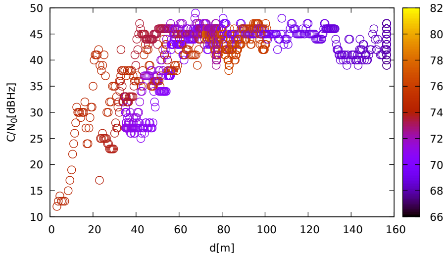
C/N_0 vs distance (ublox9 at C_2 for G11 at L1)
