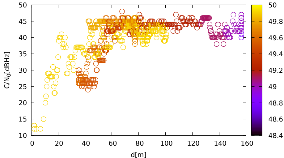
C/N 0 vs distance (ublox9 at C 2 for G14 at L1)
