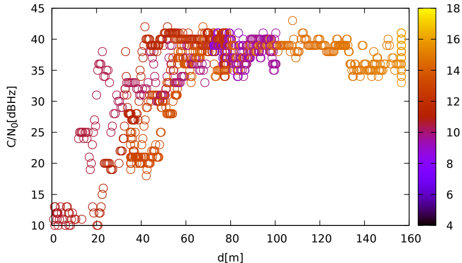
C/N 0 vs distance (ublox9 at C 2 for G17 at L1)
