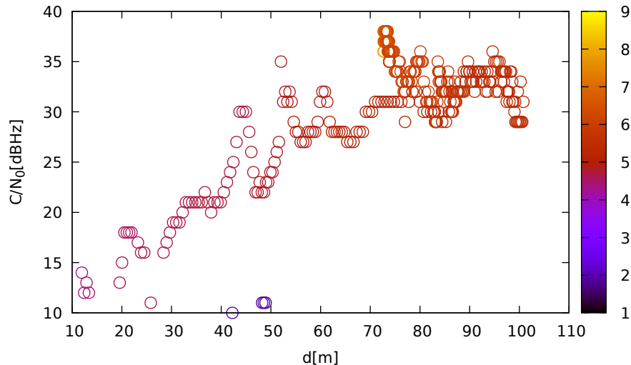
C/N 0 vs distance (ublox9 at C 2 for G21 at L1)
