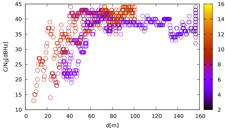
C/N 0 vs distance (ublox9 at C 2 for G27 at L1)
