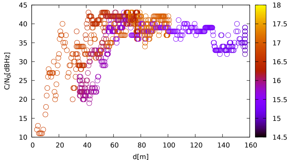
C/N 0 vs distance (ublox9 at C 2 for G28 at L1)
