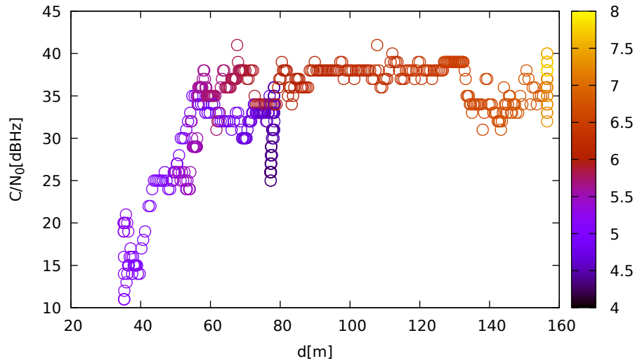
C/N 0 vs distance (ublox9 at C 2 for G31 at L1)
