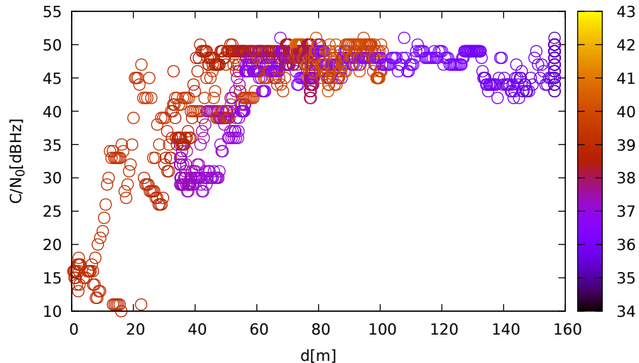
C/N 0 vs distance (ublox9 at C 2 for G32 at L1)
