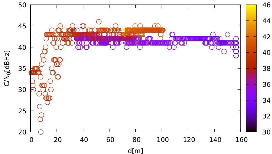
C/N 0 vs distance (ublox9 at C 2 for R06 at L1)
