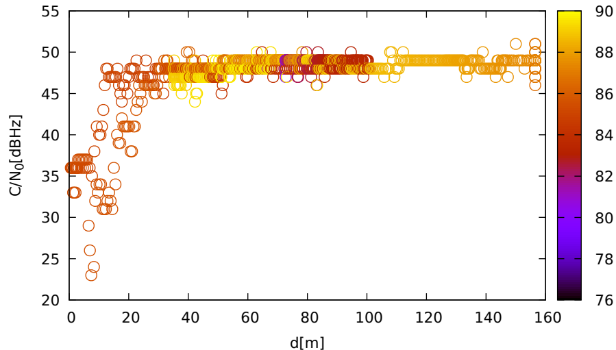
C/N 0 vs distance (ublox9 at C 2 for R07 at L1)
