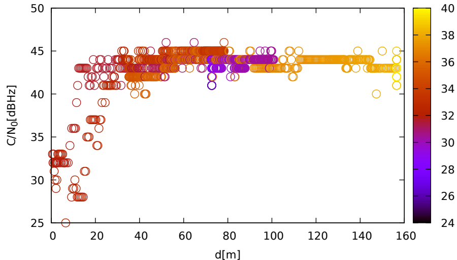
C/N 0 vs distance (ublox9 at C 2 for R08 at L1)
