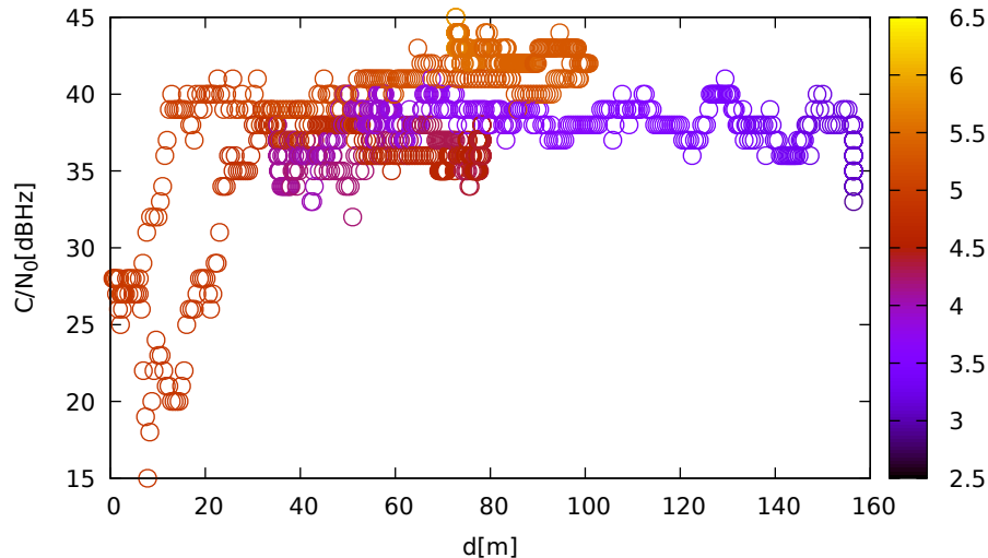
C/N 0 vs distance (ublox9 at C 2 for R14 at L1)
