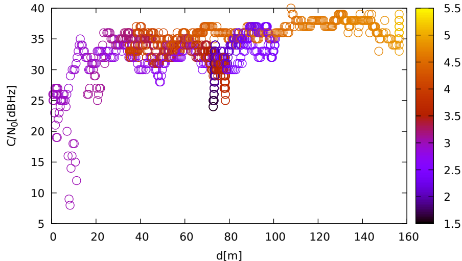
C/N 0 vs distance (ublox9 at C 2 for R15 at L1)
