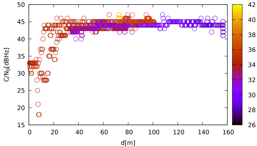
C/N_0 vs distance (ublox9 at C_2 for R21 at L1)
