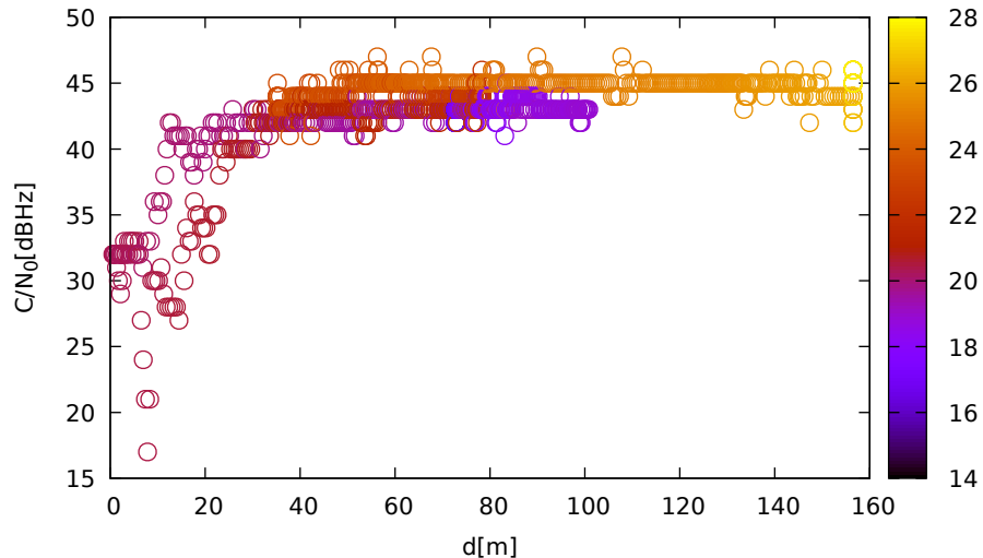
C/N 0 vs distance (ublox9 at C 2 for R23 at L1)
