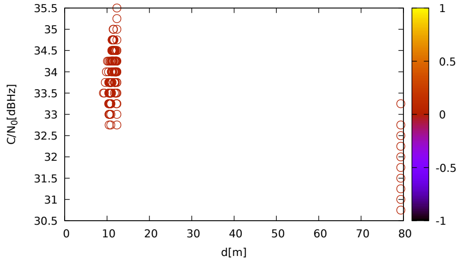
C/N 0 vs distance (JavadLSA at C 3 for C02 at L1)
