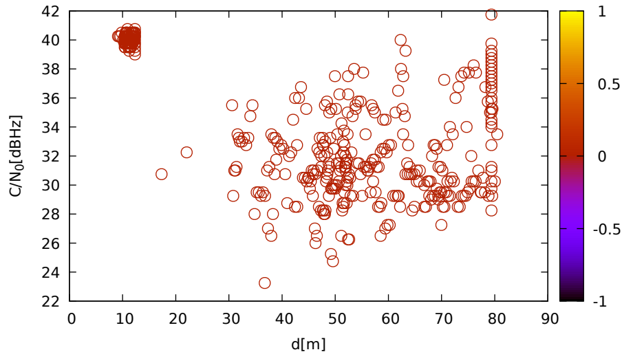
C/N 0 vs distance (JavadLSA at C 3 for C05 at L1)
