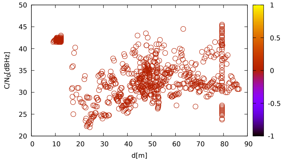
C/N 0 vs distance (JavadLSA at C 3 for C06 at L1)
