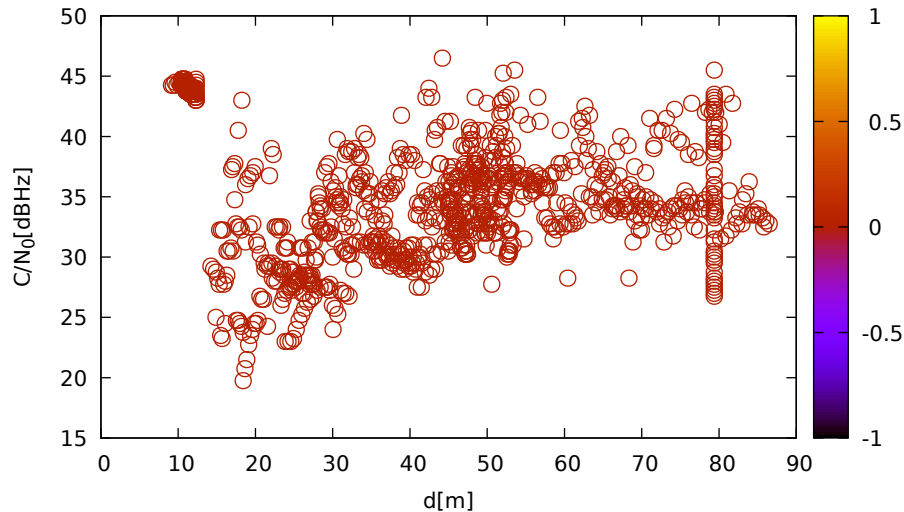
C/N 0 vs distance (JavadLSA at C 3 for C09 at L1)
