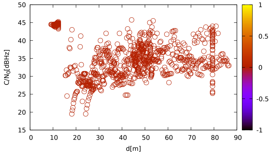
C/N 0 vs distance (JavadLSA at C 3 for C16 at L1)
