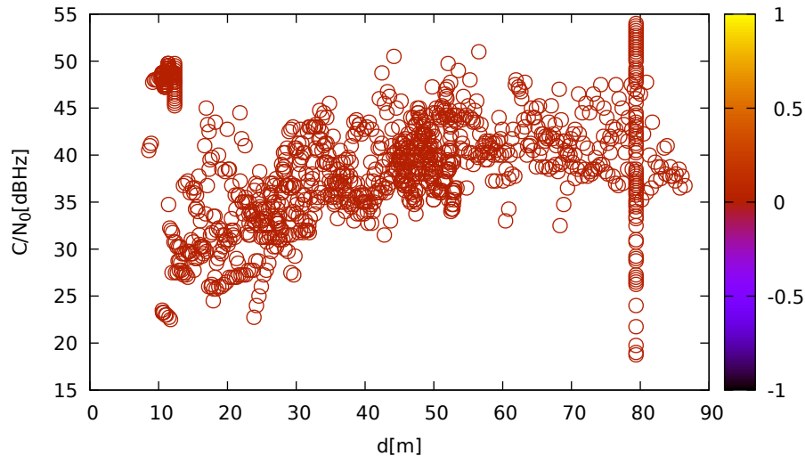
C/N 0 vs distance (JavadLSA at C 3 for C20 at L1)
