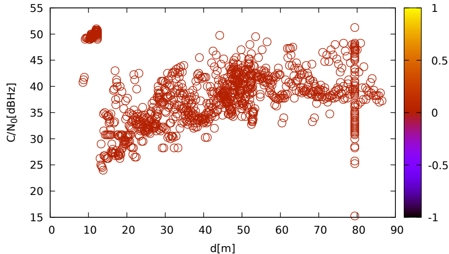
C/N 0 vs distance (JavadLSA at C 3 for C27 at L1)
