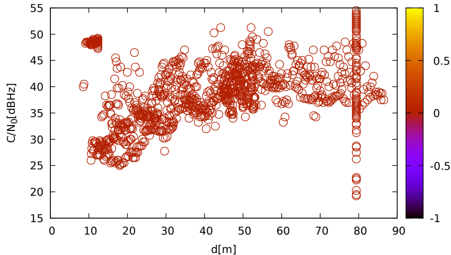
C/N 0 vs distance (JavadLSA at C 3 for C29 at L1)
