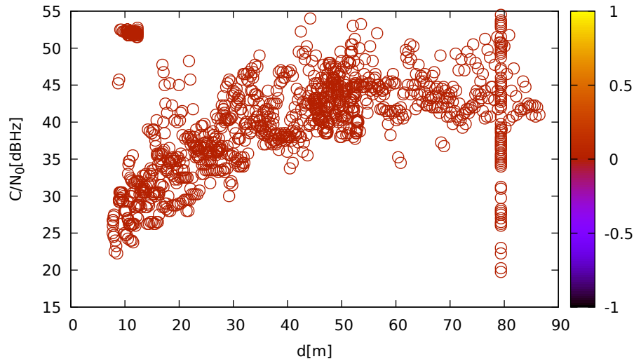
C/N 0 vs distance (JavadLSA at C 3 for C30 at L1)
