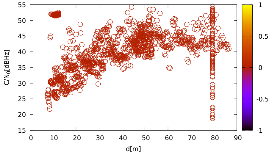
C/N 0 vs distance (JavadLSA at C 3 for C32 at L1)
