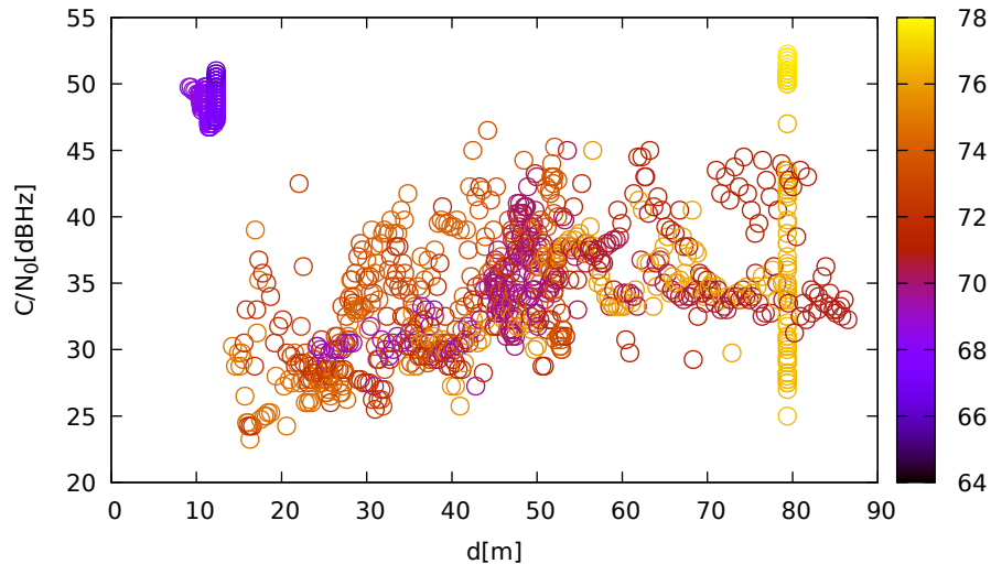
C/N 0 vs distance (JavadLSA at C 3 for G01 at L1)
