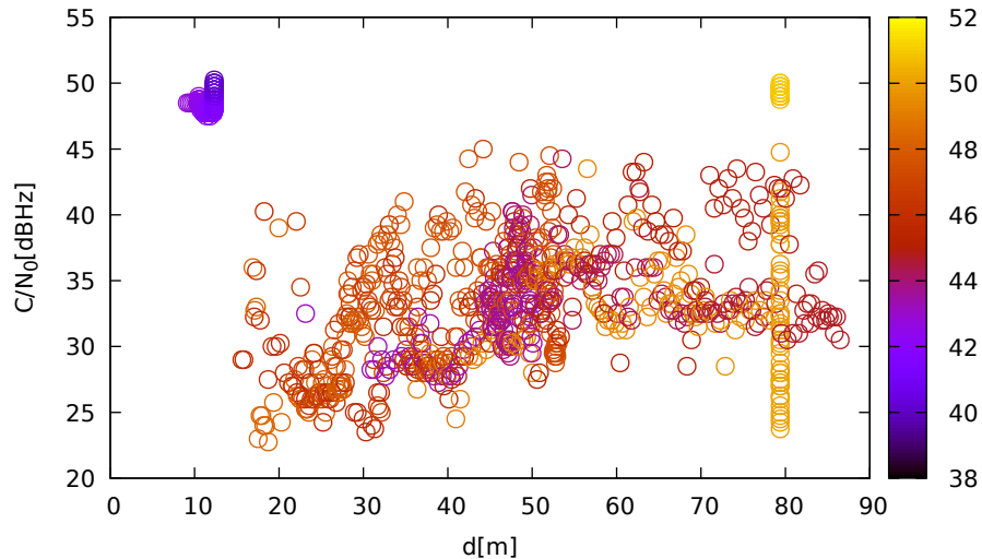
C/N 0 vs distance (JavadLSA at C 3 for G03 at L1)
