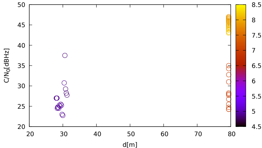
C/N 0 vs distance (JavadLSA at C 3 for G04 at L1)
